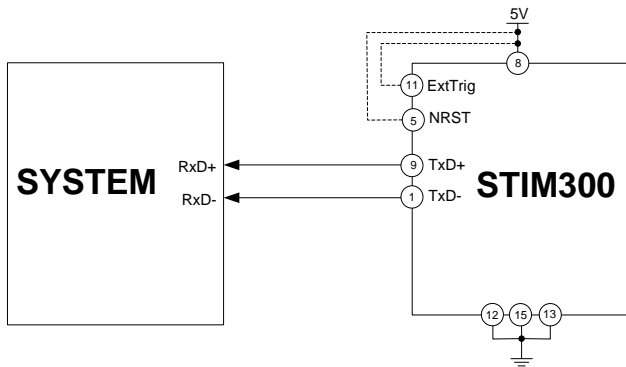
Figure 7-1: Transmit-Only Electrical Connection Diagram
