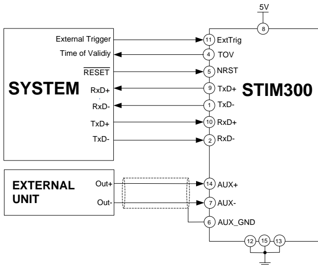
Figure 7-2: Full Function Electrical Connection Diagram
