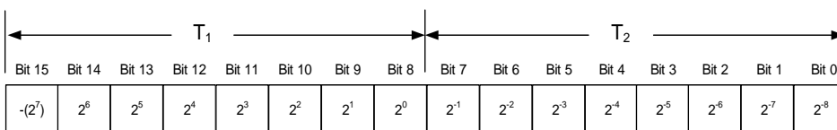
Figure 7-15: Converting temperature data to [°C]
