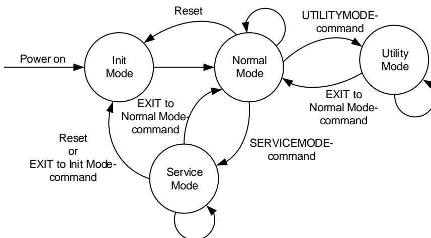
Figure 7-6: Operating modes
