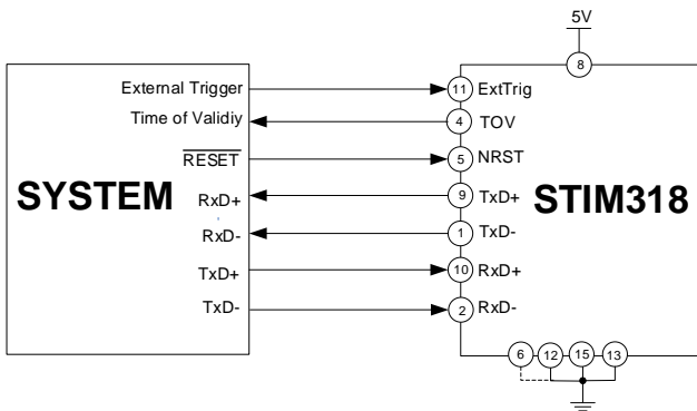
Figure 7-2: Full Function Electrical Connection Diagram
