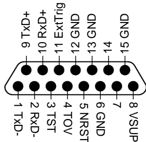
Figure 6-3: Pin configuration as seen from front of STIM318
