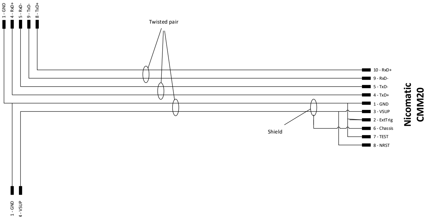
Figure 3: STIM202 EVK Wiring diagram
